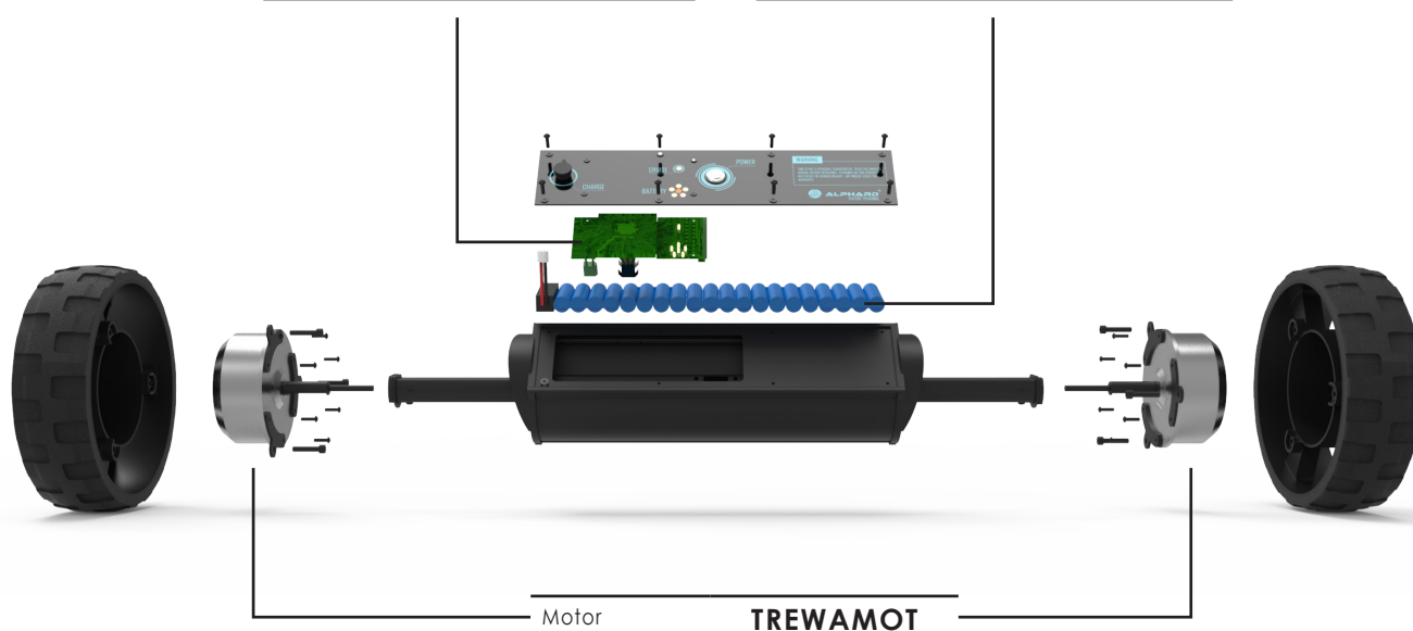
Circuit Board TREWACB
